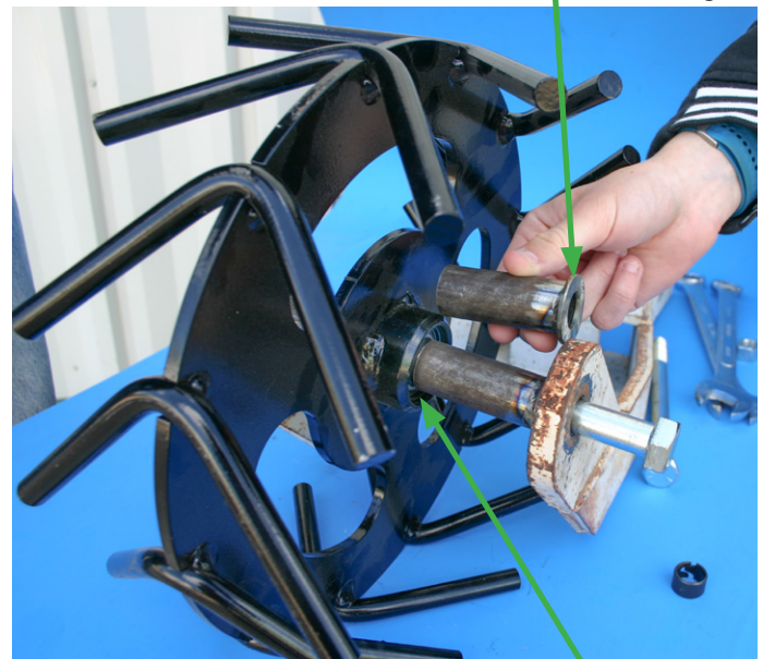
Tapered side of hub.
